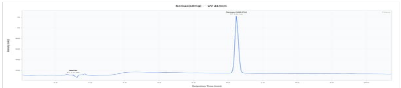
Semax 10mg - 5051: UV Chromatogram
